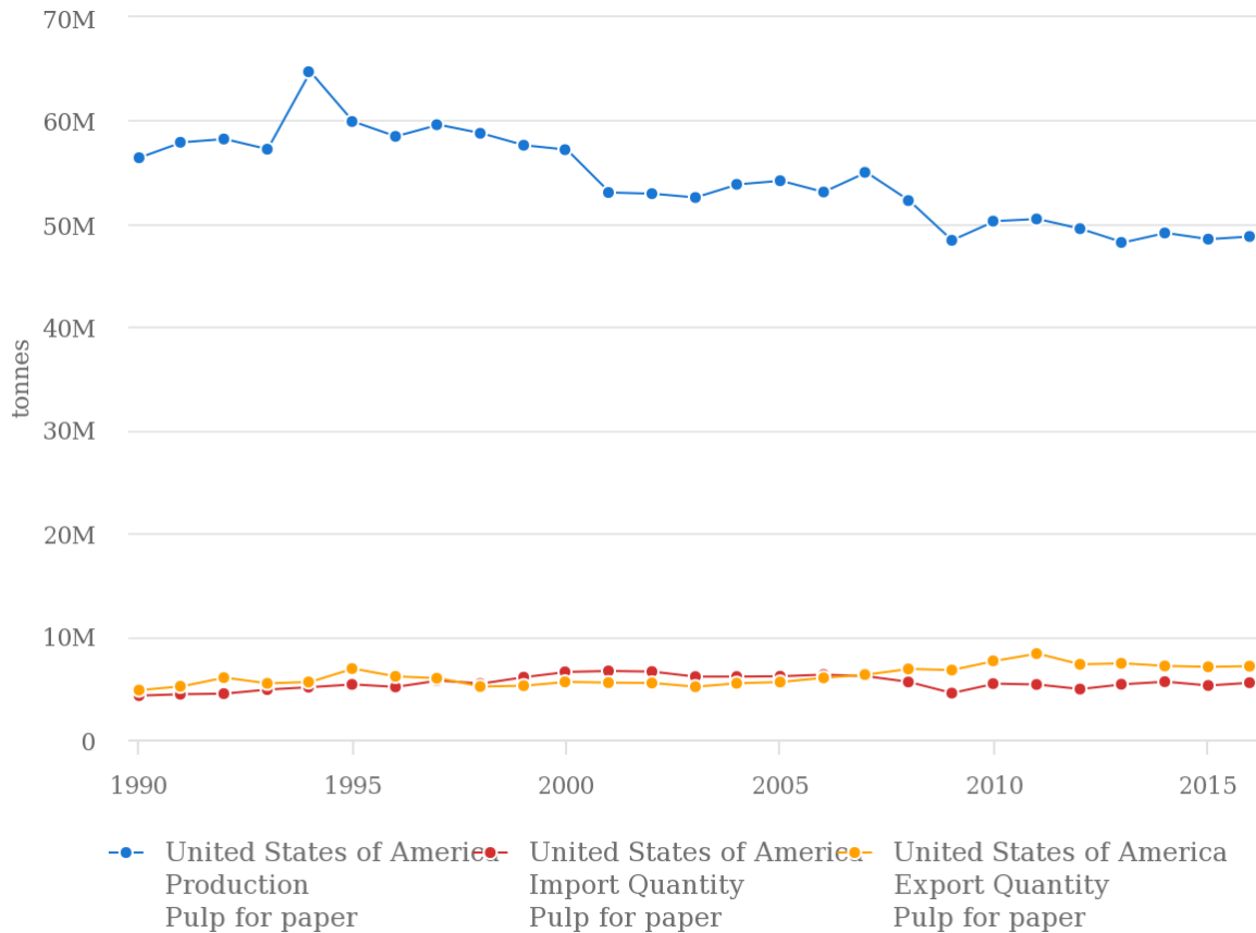
Figure 11 : Production, imports and exports of pulp and paper in the USA between 1990 and 2016 (source : FAOstat)
