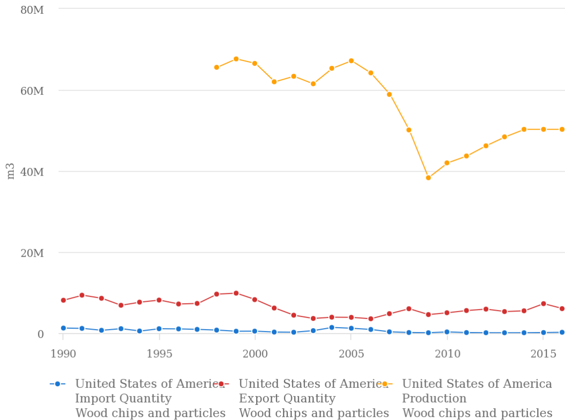
Figure 12 : production, imports and exports of chips and particles in the USA between 1990 and 2016 (source : FAOstat)
